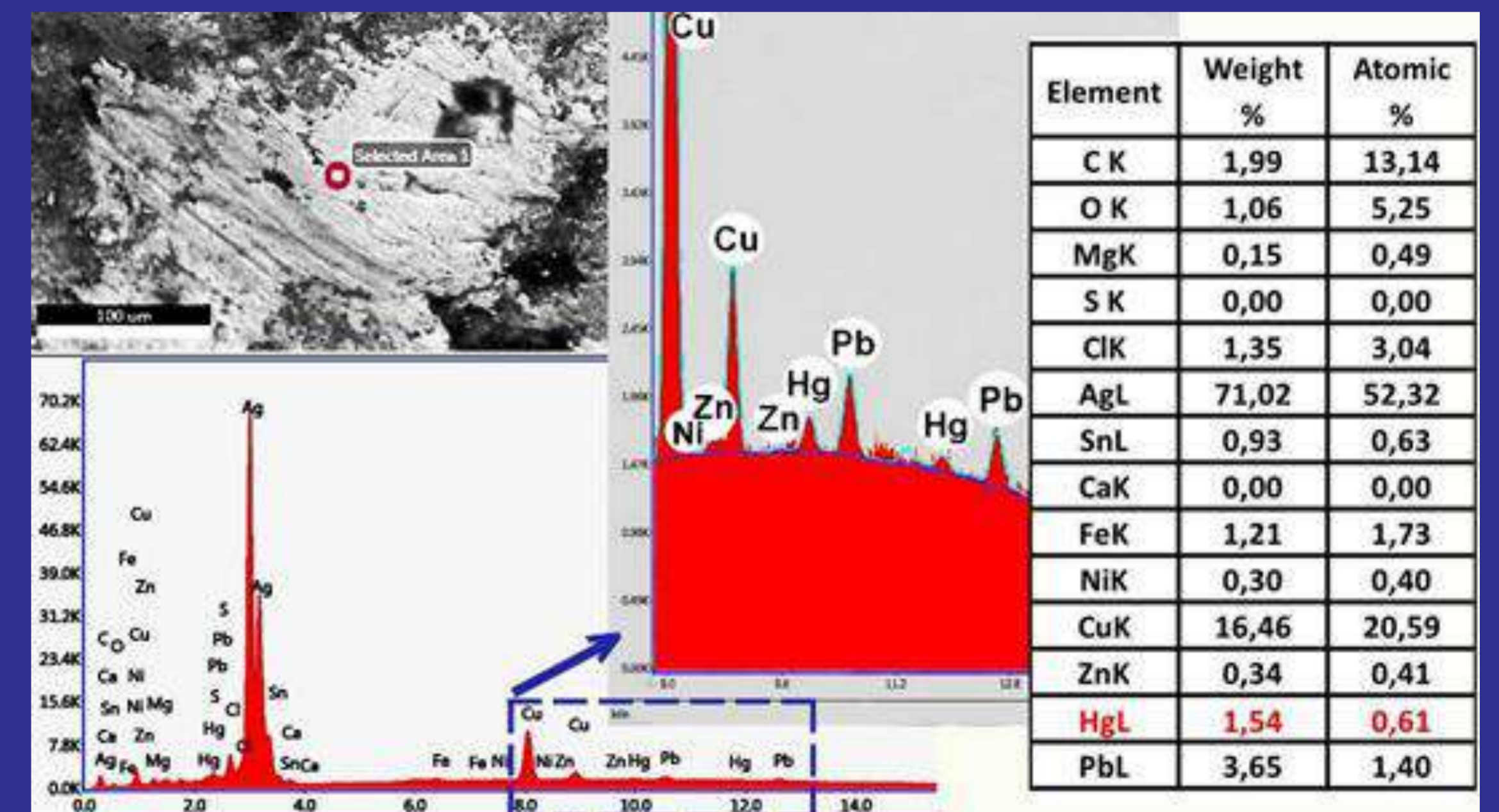
Scanning Electron Microscopy - Energy Dispersive X-ray Microanalysis (SEM-EDXM) technique: chemical element Hg was detected in the upper silver layer of coins, the silvering procedure using Hg-Ag amalgam has been identified
